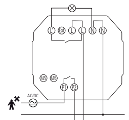
SPHINX 104-360/2 AP, SPHINX 104-360/2
